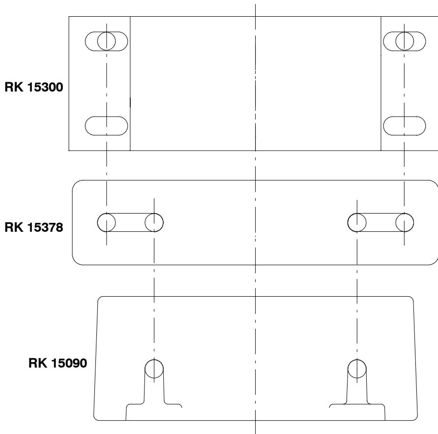
Mounting comparison with bracket centerline at the same location.
