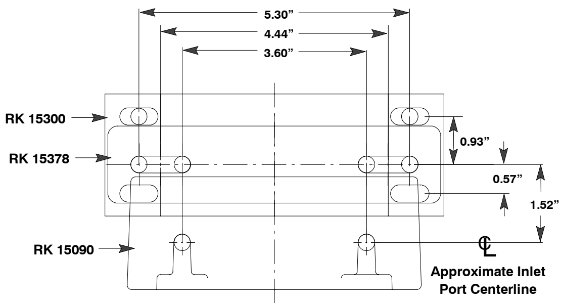
Bracket comparison with filter port centerline at the same location.
