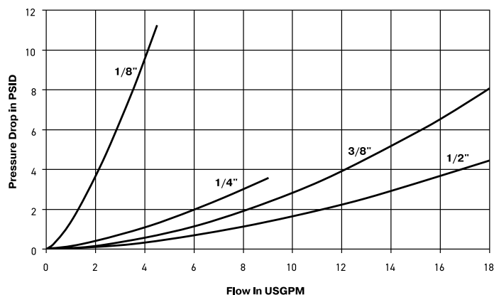
ST Series (1/8", 1/4", 3/8", 1/2") Test Fluid: Oil - 150 SUS
