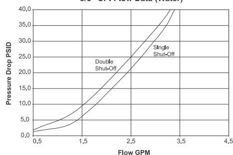
3/8" CPI Flow Data (Water)
