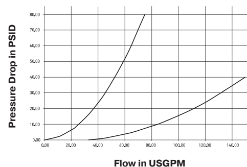
59 Series (1" & 1-1/2") Test Fluid: Oil - 150 SUS
