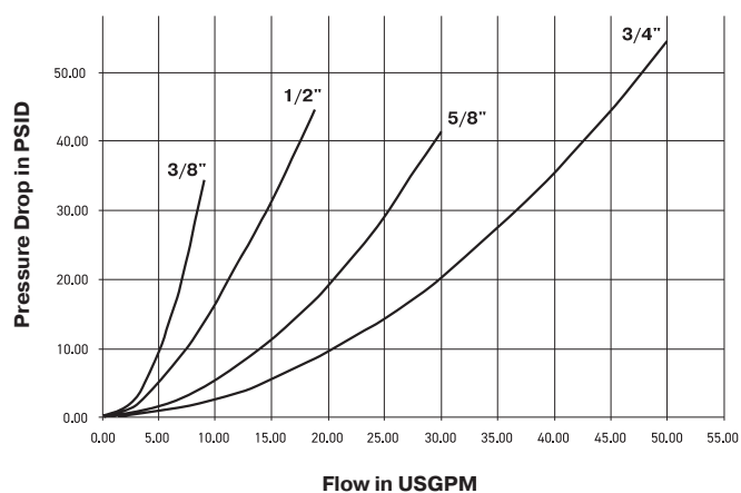
FET Series (3/8", 1/2", 5/8" & 3/4") Test Fluid: Oil - 150 SUS)
