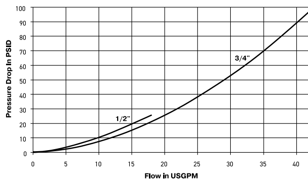
6100 Series (1/2" & 3/4") Test Fluid: OIL 150 SUS
