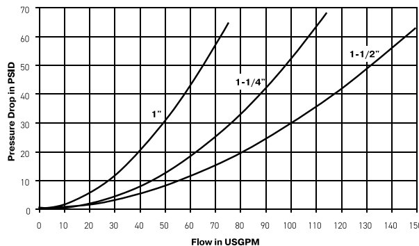
6100 Series (1", 1-1/4", 1-1/2") Test Fluid: OIL 150 SUS
