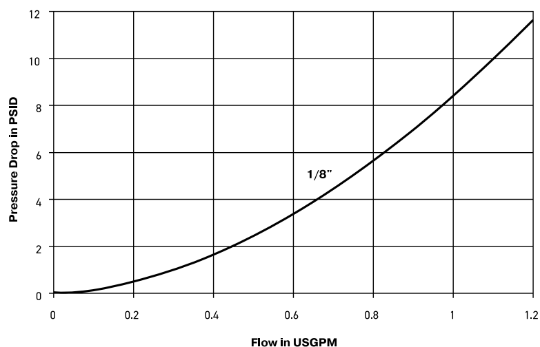
Rectus 21 DSO Series Test Fluid: Water
