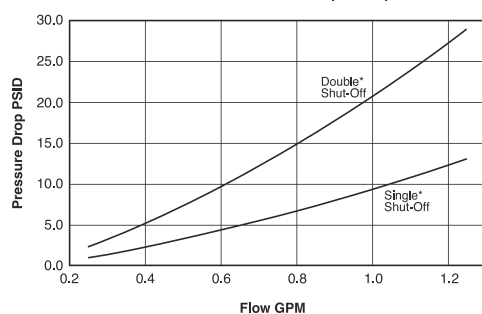
1/4" CPI Flow Data (Water)
