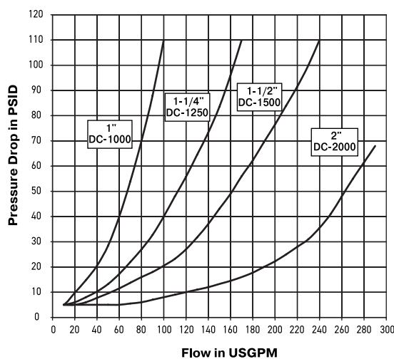
DC Series (1", 1-1/4", 1-1/2" & 2") Test Fluid: Oil - 200 SUS
