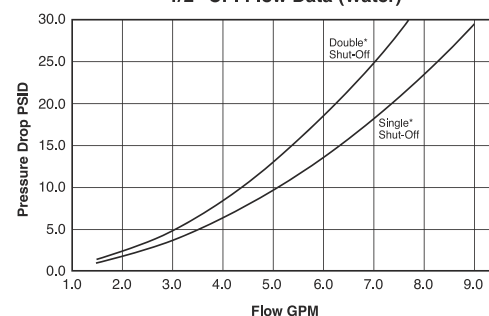
1/2" CPI Flow Data (Water)
