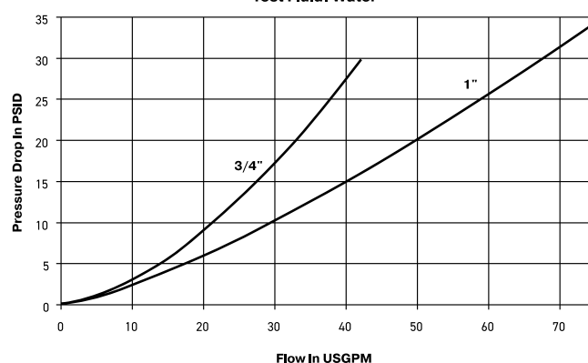
FS Series (3/4" & 1") Test Fluid: Water
