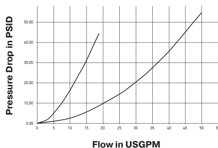
59 Series (1/2" & 3/4") Test Fluid: Oil - 150 SUS
