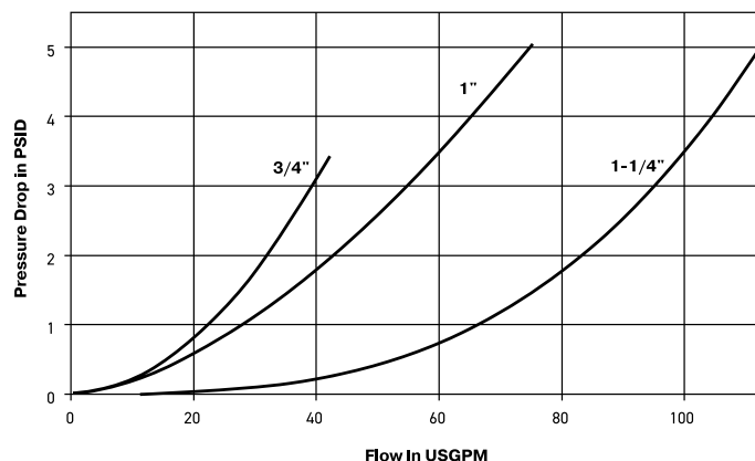
ST Series (3/4", 1", 1-1/4") Test Fluid: Oil - 150 SUS
