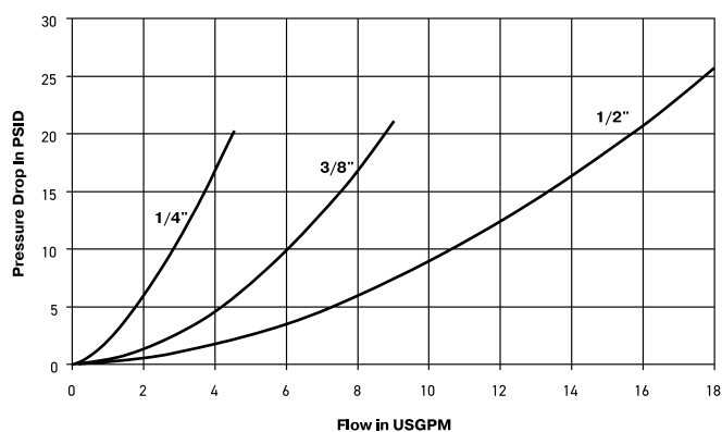
FS Series (1/4", 3/8", 1/2") Test Fluid: Water
