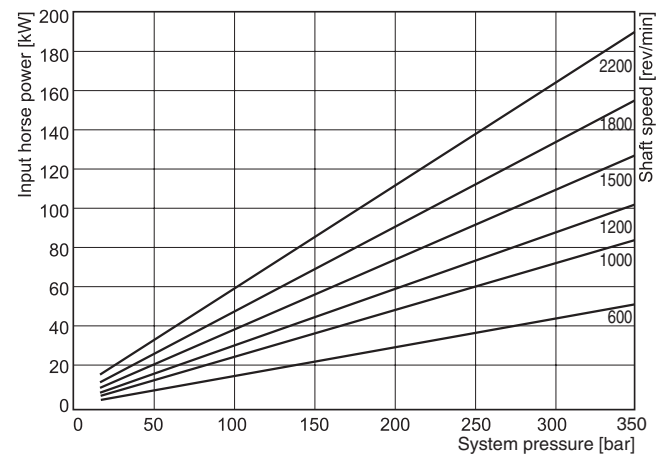
P2145 Input power - full stroke
