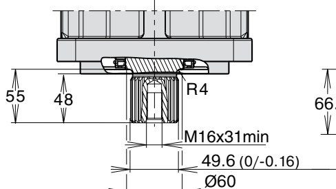
Type D spline shaft W50x24x9g DIN 5480 side fit
