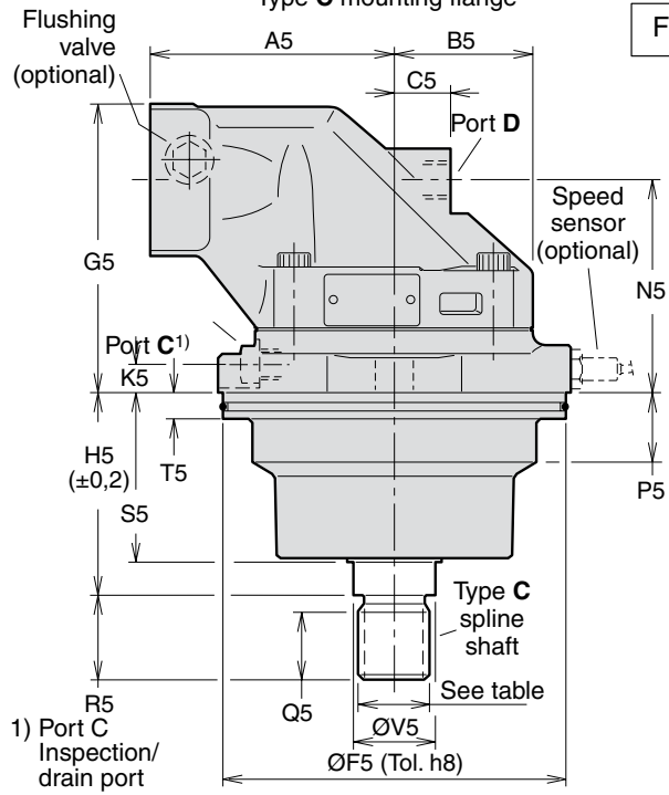
Type C mounting flange
