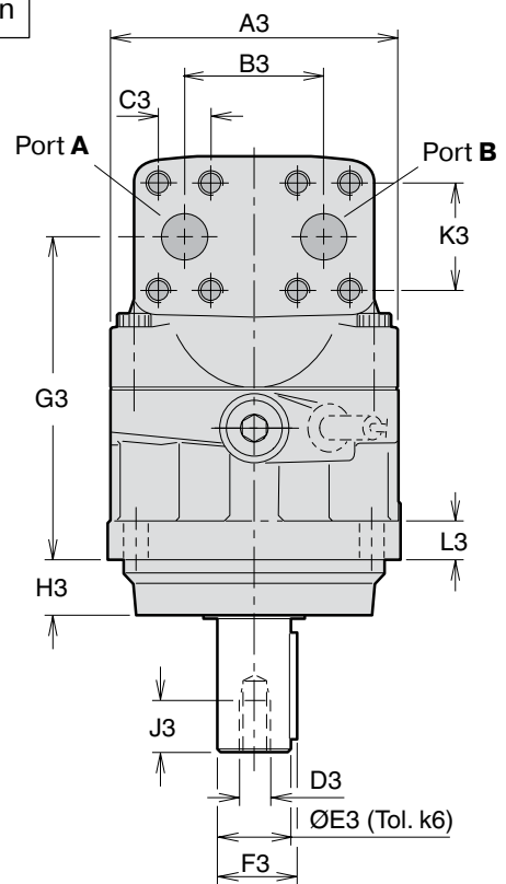
Shaft option V (F12-40)
