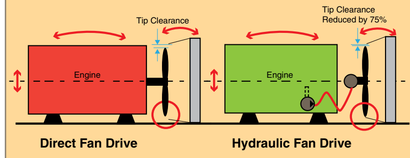
A hydraulic fan drive reduces tip clearance and improves airflow by 10-15%.
