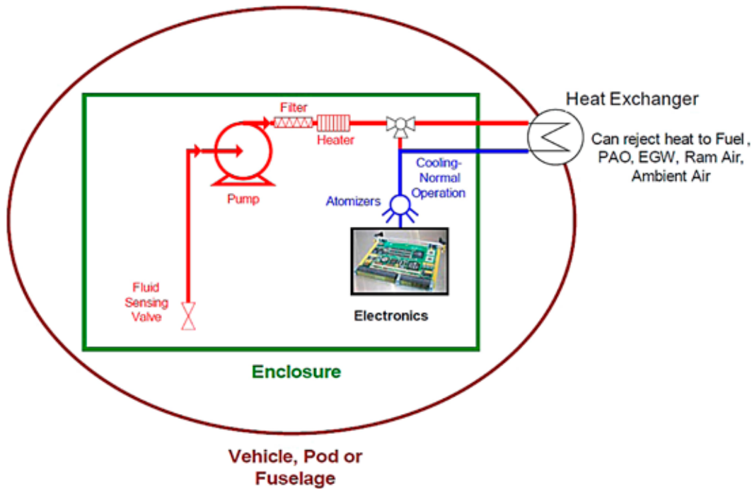
FIGURE 1. SYSTEM DIAGRAM OF DIRECT SPRAY ENCLOSURE
