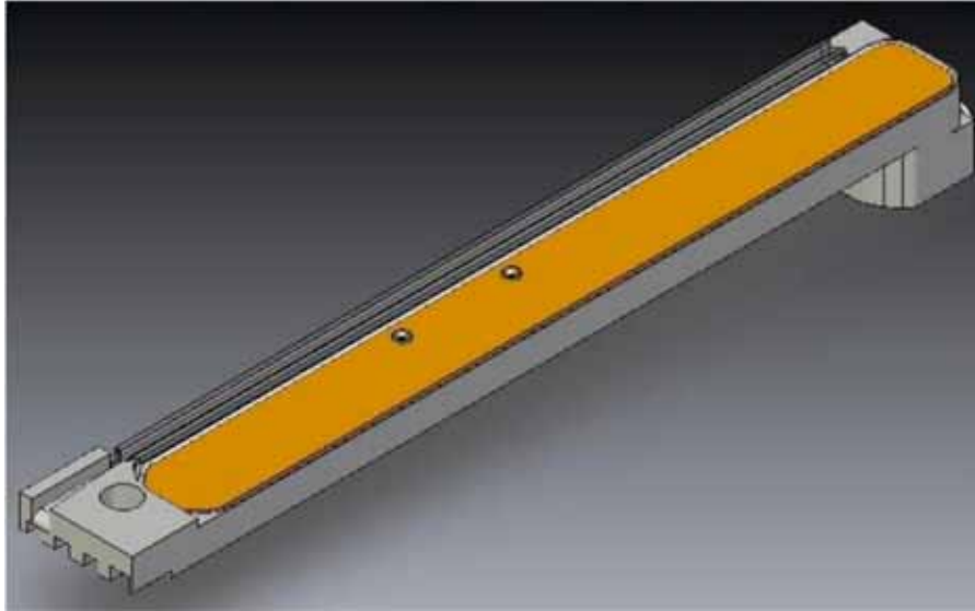
FIGURE 2. SPRAY MANIFOLD WITH INTEGRATED CARD GUIDE
