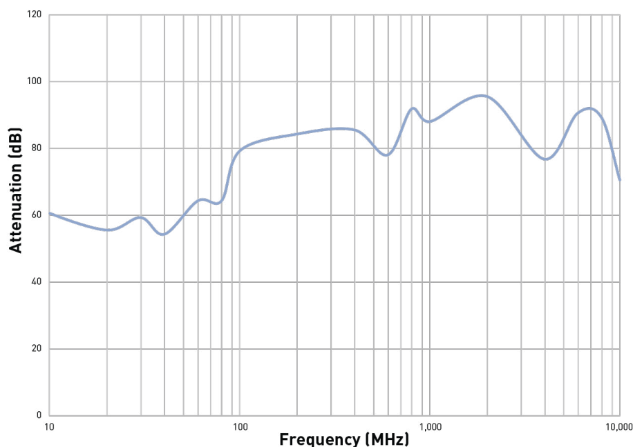
Figure 1 Shielding Effectiveness for CHO-SHRINK 1061, 1/2" diameter tubing
