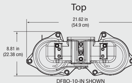
DFBO-10-IN SHOWN
