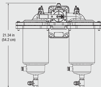
DFBO-10-IN SHOWN Front
