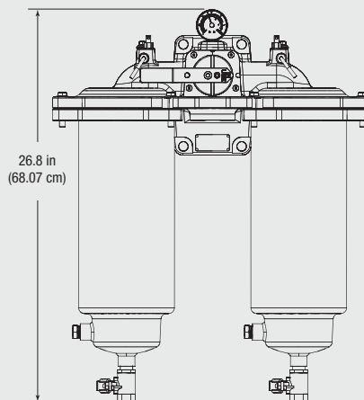
DFBO-14-MA SHOWN Front
