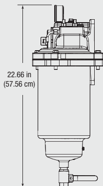
DFBO-10-MA SHOWN Profile
