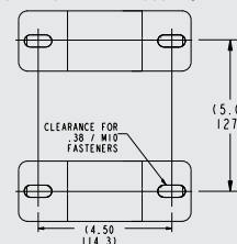
MOUNTING PATTERN 1000MA/MAM
