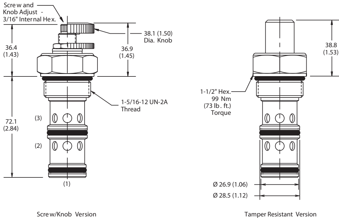
Screw/Knob Version
