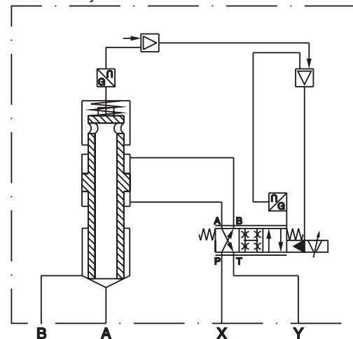
Function Symbol
