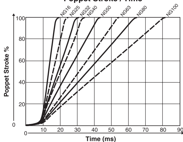
Poppet Stroke / Time
