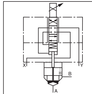
Function Symbol
