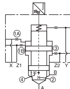
Position control
