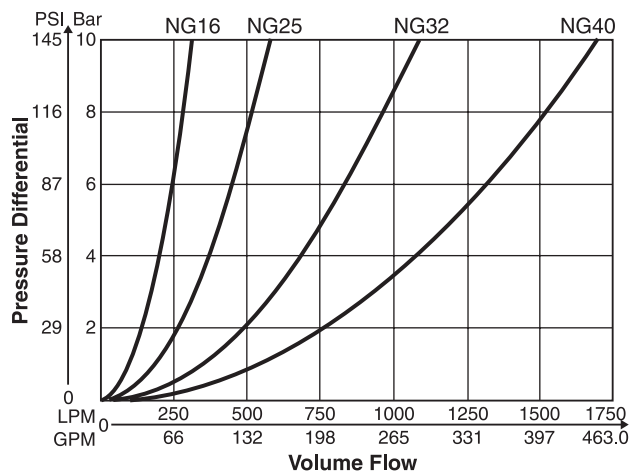
Poppet 08*
