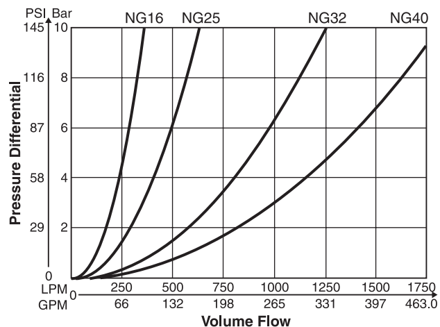
Poppet 01, 04, 07*
