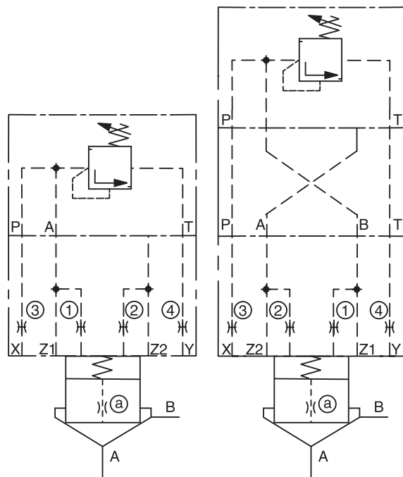
NG16 - NG40
