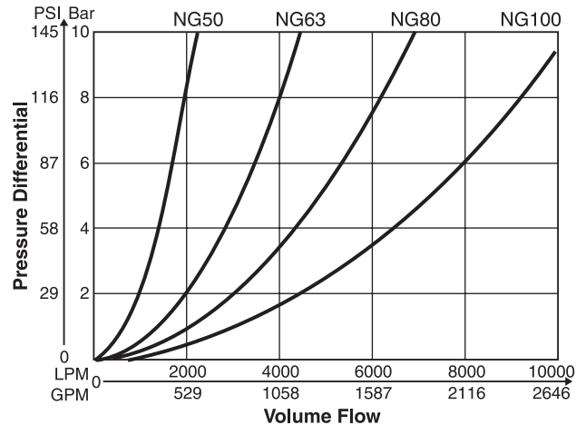
Poppet 08*
