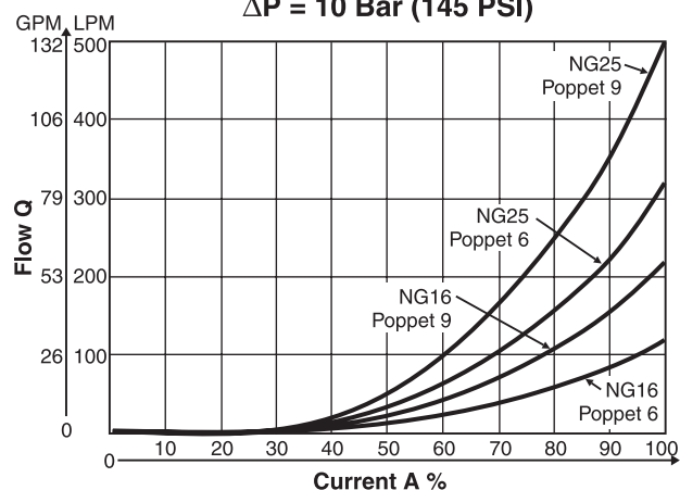
NG16 and NG25 Solenoid Current \Delta P = 10 \text{ Bar (145 PSI)}
