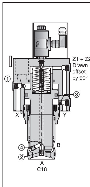
Position control
