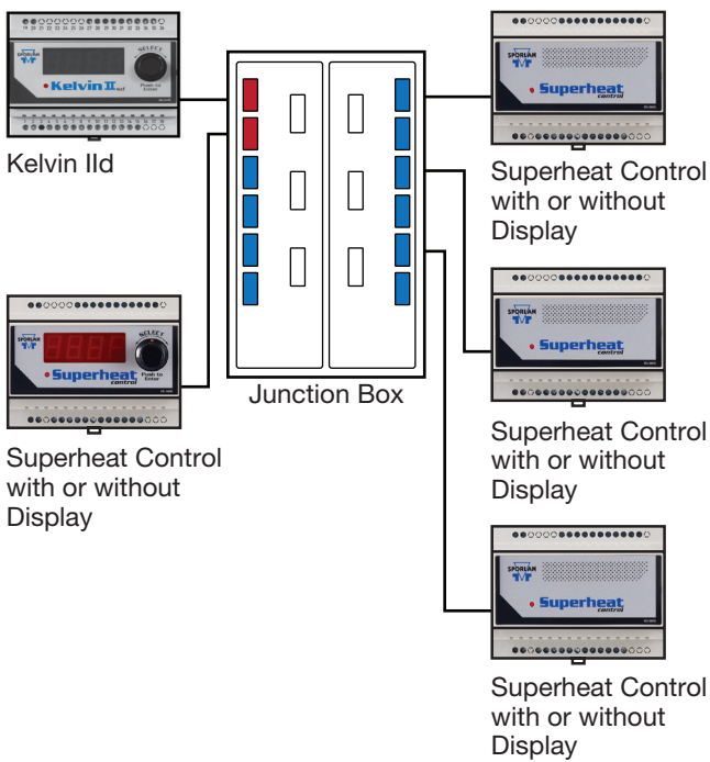
Figure 3 - Display Networking
