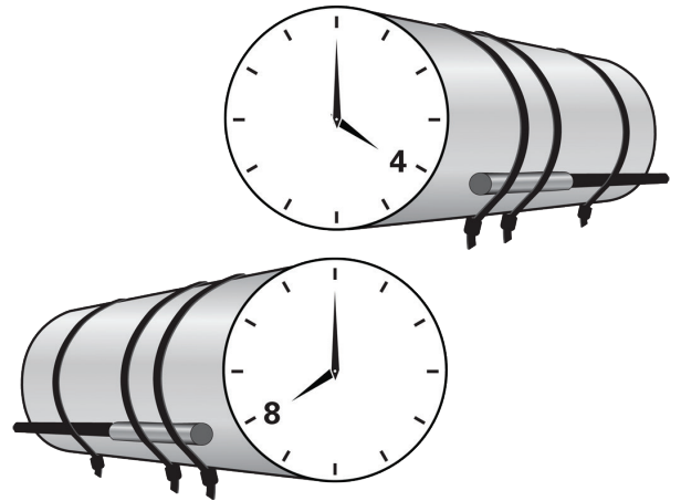
Figure 8 - Temperature Sensor Positioning
