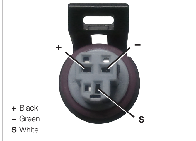
Figure 7 - Pressure Sensor Cable
