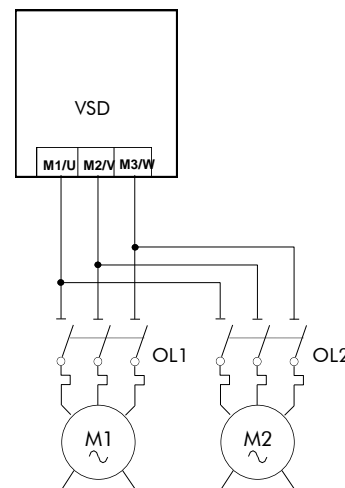
Figure Chapter 10 -1 Single Drives supplying multiple Motors
