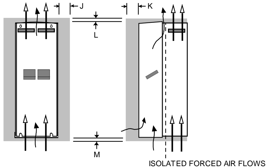
Figure Chapter 3 -10 Air Clearance for a Cubicle-Mount Product/Application
