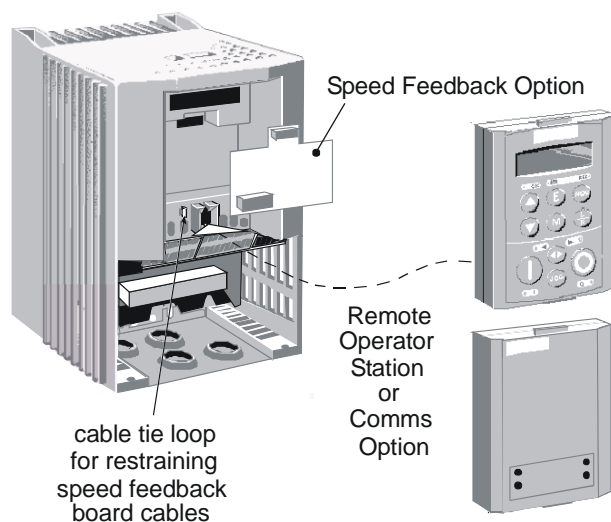
Frame B illustrated
