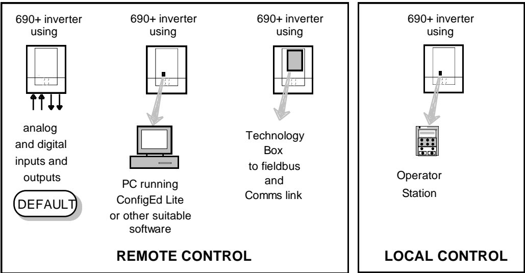
Frame B illustrated
