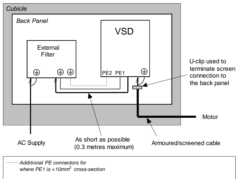
Figure Chapter 9 -1 EMC and Safety Earthing Cabling
