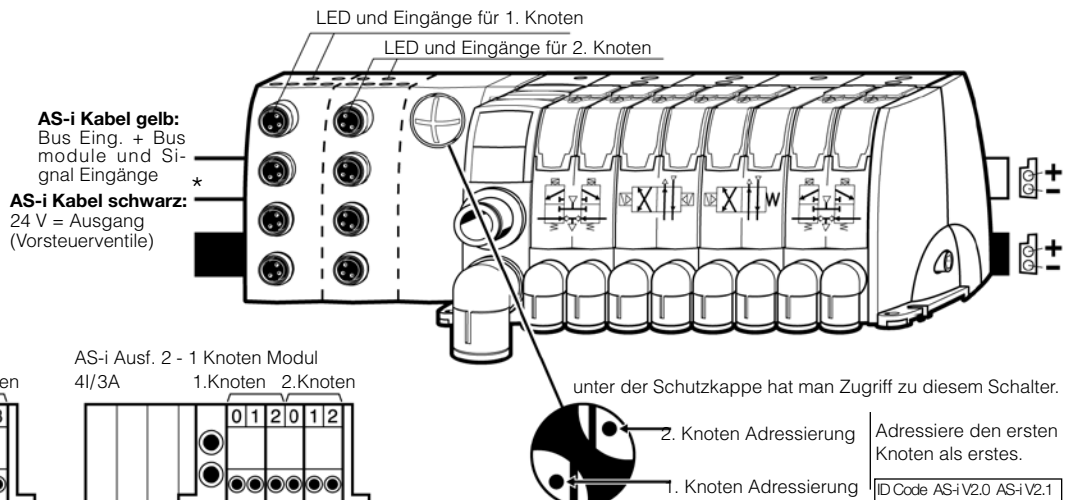
AS-i Standard 2 Knoten Modul
