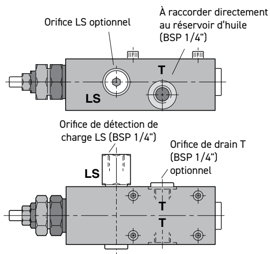
Orifices de commande LS.
