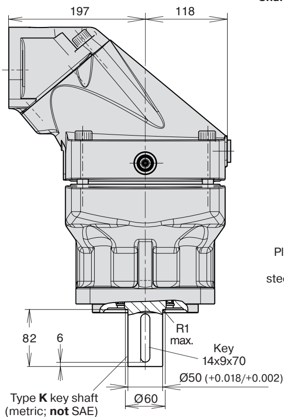
Shaft option K
