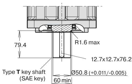
Shaft option T
