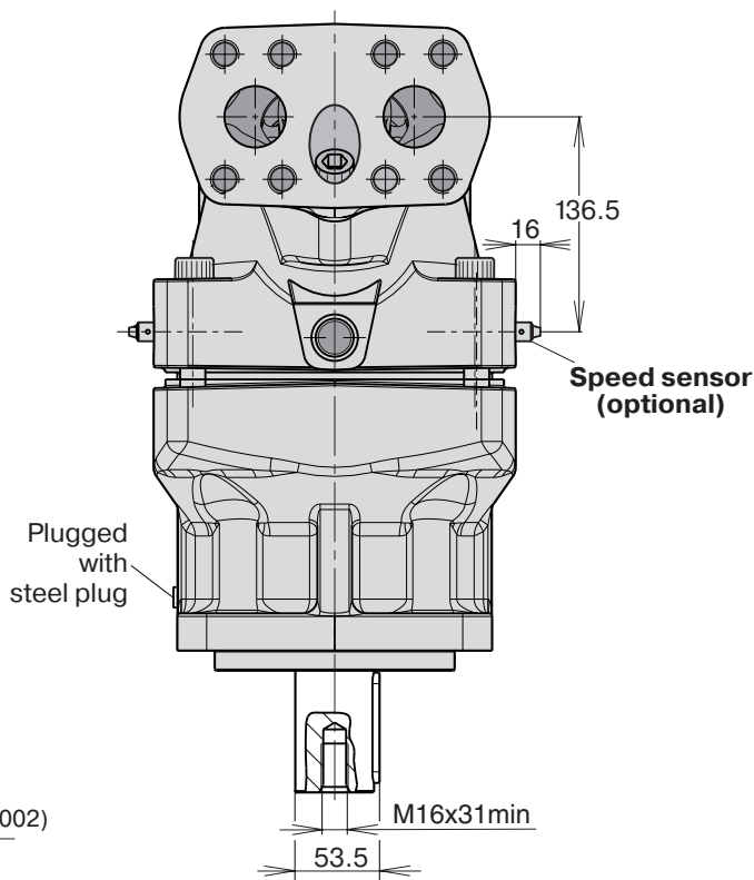
Shaft option K
