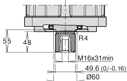
Shaft option D
