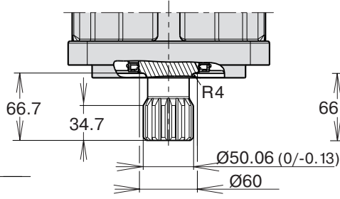
Shaft option F
