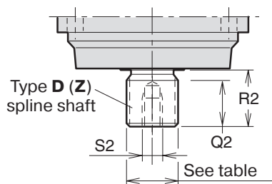
Shaft option D (Z)
