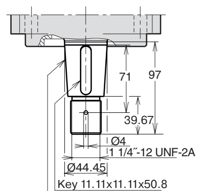
Tapered key shaft "V" SAE J744 44-3 (D&E)
