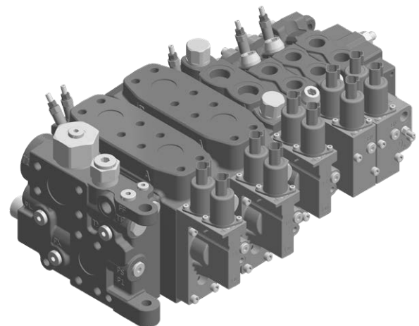
VA450+VA300+VA130 combination valve.
