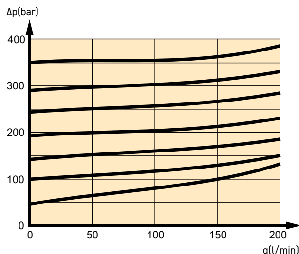
Pressure relief characteristics PA
