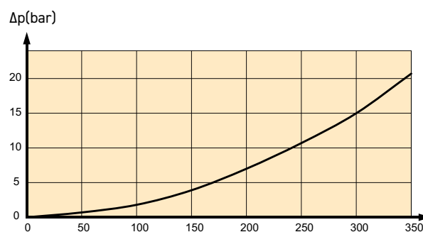
PA, PAU, N2 - Anti-cavitation characteristics (x2)
