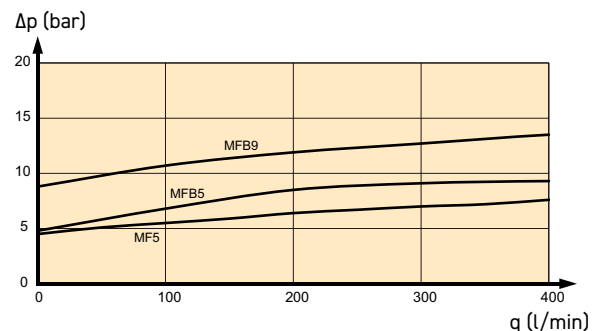
MF5, MFB5, MFB9 - Counter pressure characteristics
