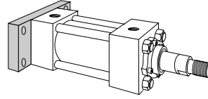
Rectangular Flange/Cap End Model 62 (NFPA MF2)
