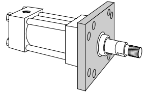
Square Flange/Head End Model 65 (NFPA MF5)
