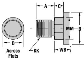
Style No. 2-Standard Threaded on Turndown Section
