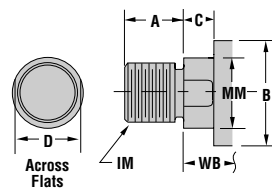
Style No. 5 Threaded Intermediate Male
