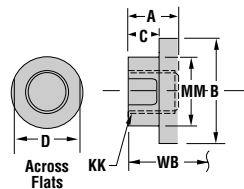
Style No. 4 Short Rod End-Internal Threads
