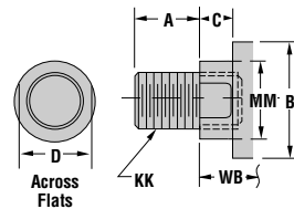
Style No. 6 Studded Rod End (Available Thru 2" Rod Diameter)
