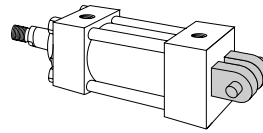
Fixed Clevis Model 84 (NFPA MP1)
