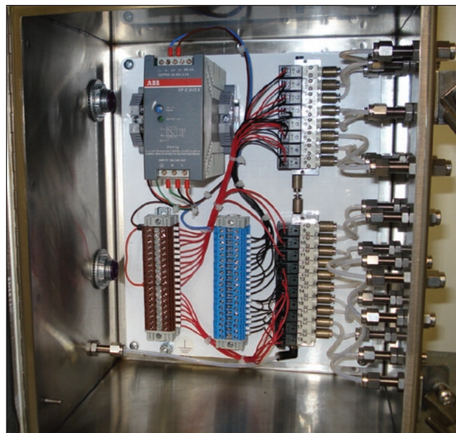
Pilot Pro™ Analog Enclosure – Customer Application Example
