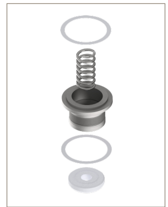
Bellow & Seal Kit for Parker Bestobell Cryogenic Pressure Regulators
