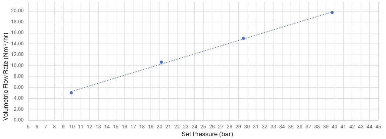
DN6 CSRV Flow Rate vs Set Pressure
