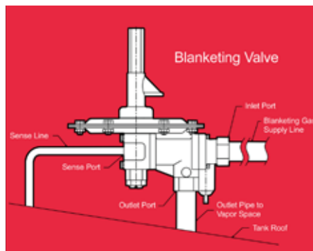
A tank blanketing valve controls the flow rate of nitrogen based on pressure. Source: Protectoseal
