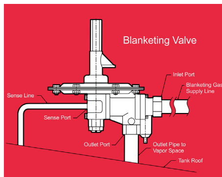
A tank blanketing valve controls the flow rate of nitrogen based on pressure. Source: Protectoseal
