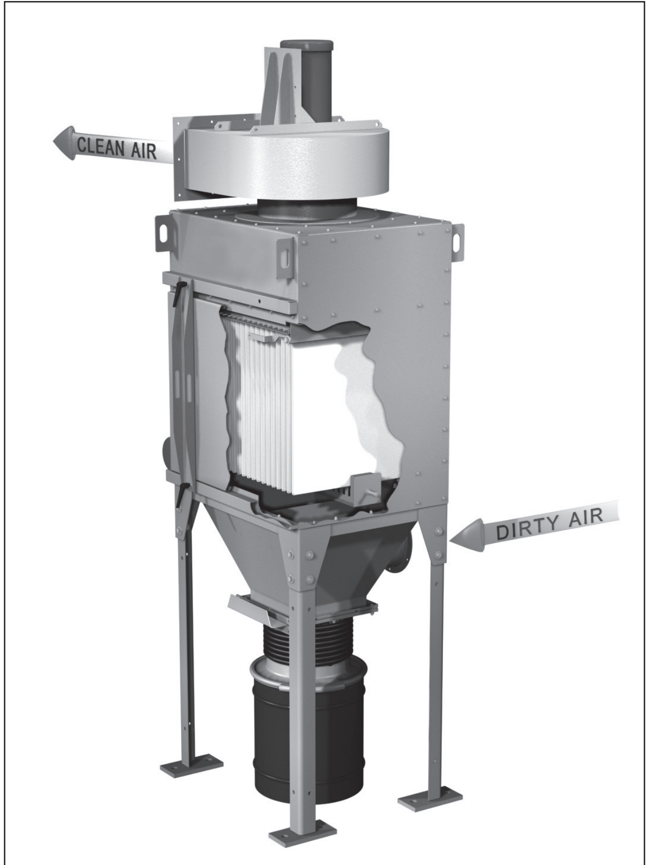
Figure 1. Unit Operation
