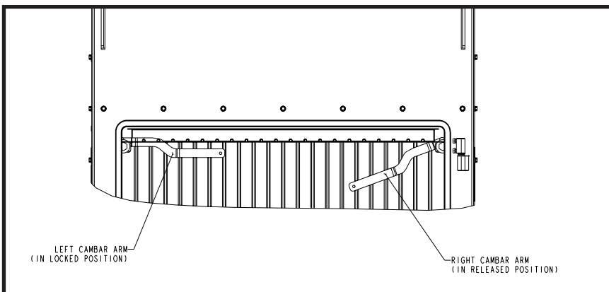
Figure 11. Filter Sealing Mechanism
