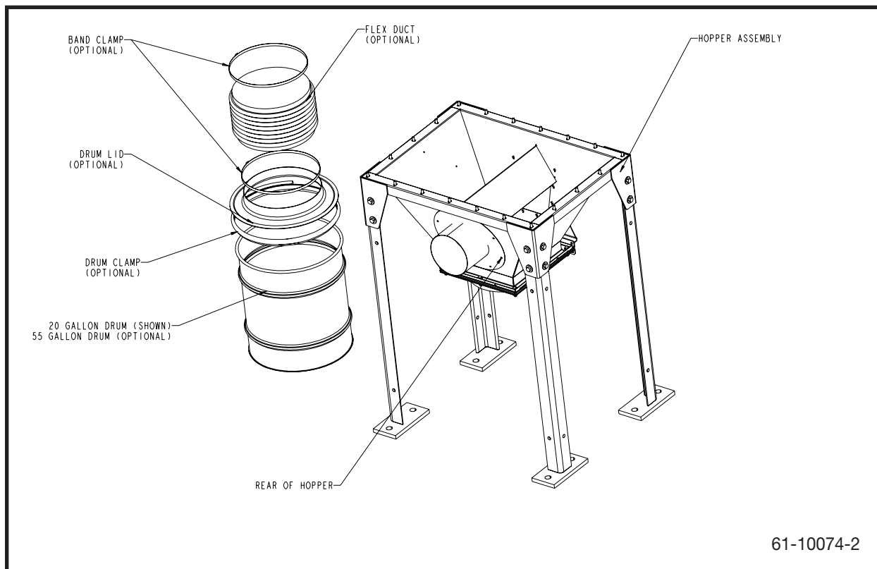
Figure 3. Drum Assembly
