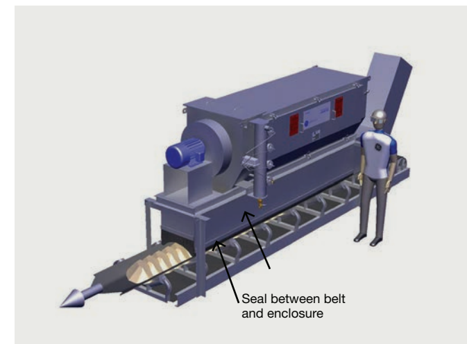
Figure 32. Point venting a belt conveyor with a horizontal collector.
