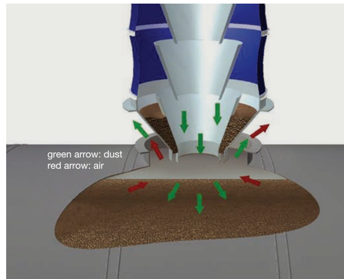
Figure 27. Typical truck loading spout.
