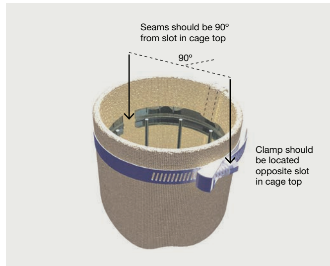
Figure 10. Correct positioning for bottom-load bags. Snapband bags for top-access pulse-jet units should also be installed with the seams facing in the same direction to make it easier to identify and troubleshoot problem areas.
