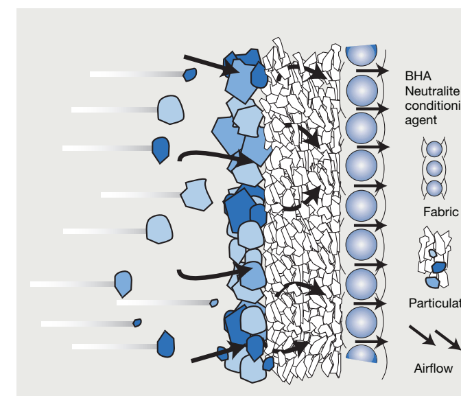
Figure 24. By injecting an initial dust cake of conditioning agent, the fabric is protected from particulate, while still allowing airflow to pass through the dust cake.
