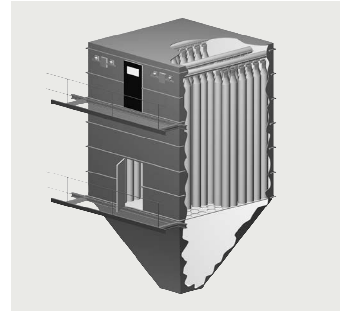
Figure 18. Dust collector system using shaker cleaning.
