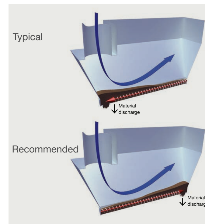
Figure 22. Recommended screw conveyor direction.
