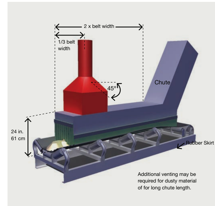
Figure 2. Improved belt conveyor hooding.*
