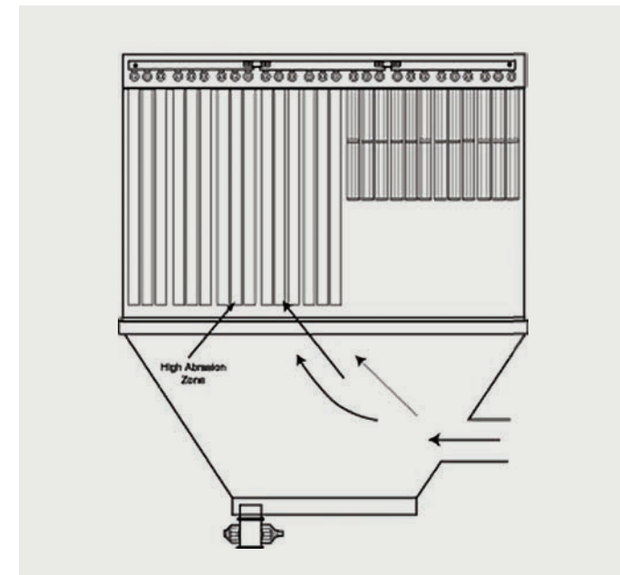
Figure 37. The shorter length of pleated filter elements helps reduce abrasion problems.
