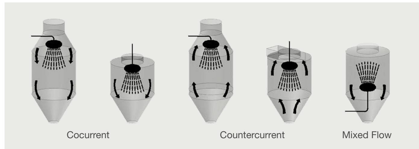
Figure 41. Spray drying flow patterns.
