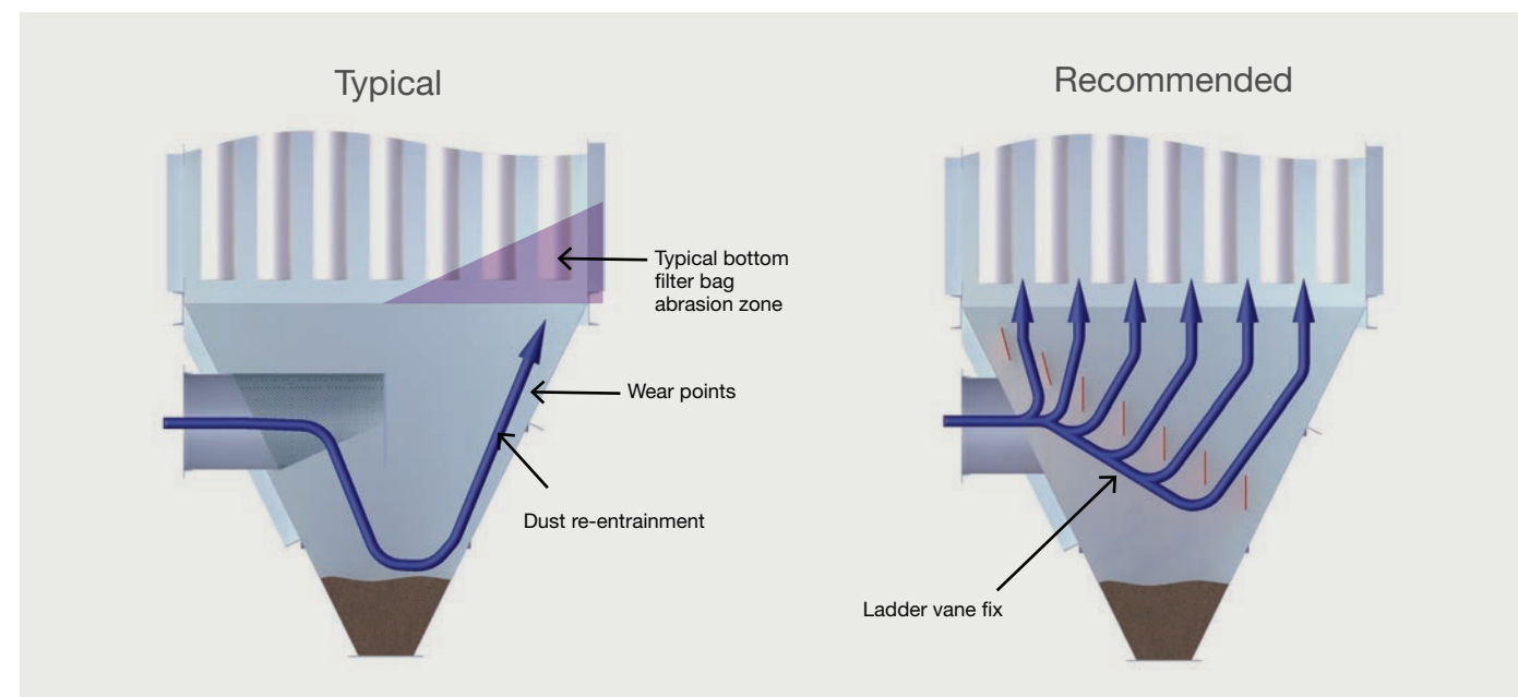
Figure 23. Properly dispersed air reduces abrasion.
