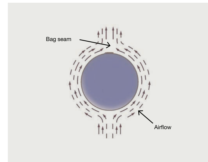
Figure 8. In pulse-jet collectors, all bag seams should face the same direction.
