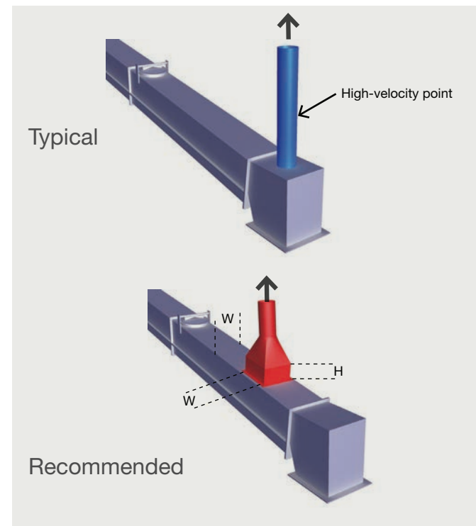
Figure 4. Hood fix for air conveyor.*
