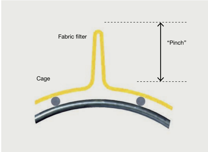
Figure 12. “Pinch” is calculated by subtracting the actual cage circumference from the bag circumference, then dividing the result by 2.
