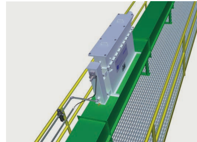
Figure 30. Air conveyor vent collector mounted on air slide.
