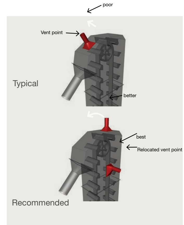
Figure 5. Improved elevator vent placement.*
