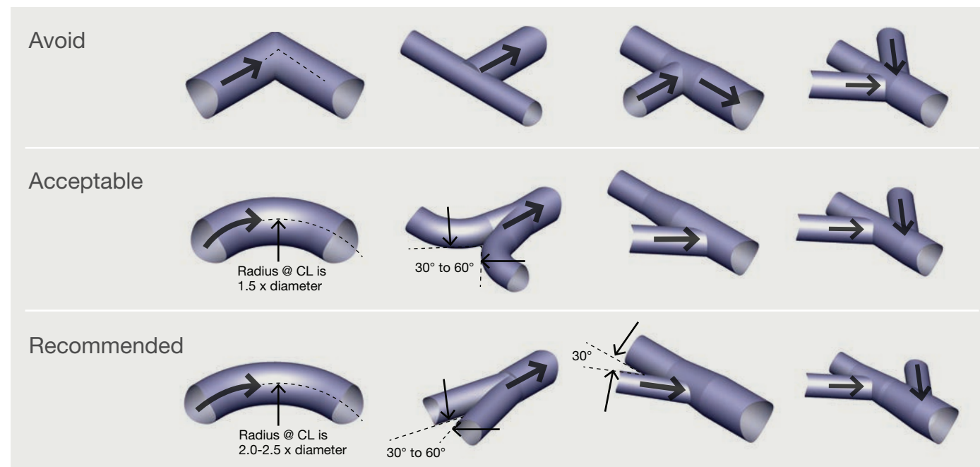
Figure 1. Elbow, joint and branch duct designs that promote efficient airflow.*
