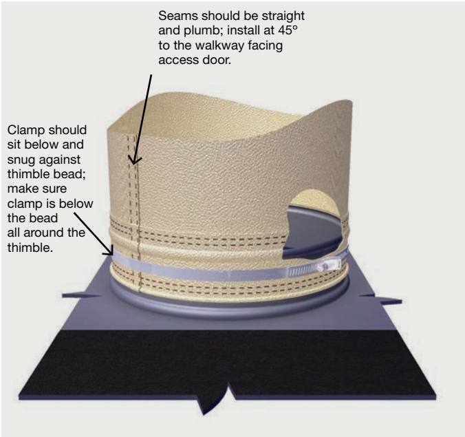
Figure 17. Important bag installation checkpoints.
