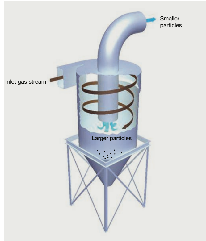
Figure 20. A cyclone precollector.
