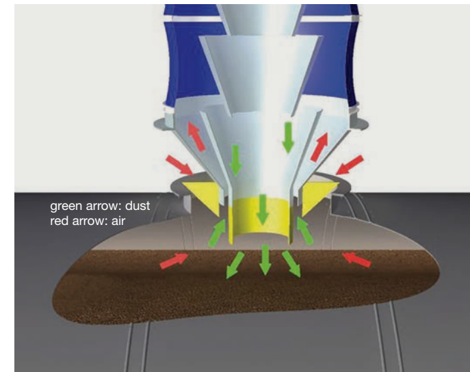
Figure 28. Recommended truck loading spout.
