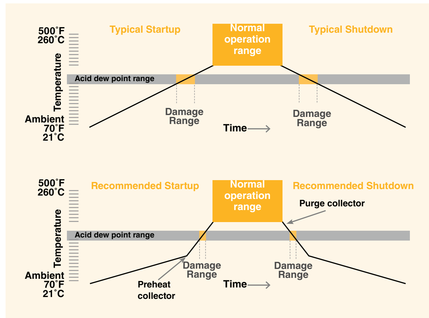
Figure 40. Startup/shutdown timeline in relation to dew point.
