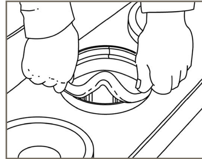
Figure 11. To properly install a snapband filter bag, bend the snapband into a kidney shape and place the grooved gasket into the tubesheet hole, positioning the seam first. Let the snapband expand into place. You should hear a sharp popping noise when the band is properly seated around the circumference of the tubesheet hole.
