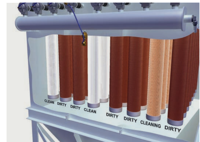
Figure 7. Recommended pulse-jet row cleaning sequence.
