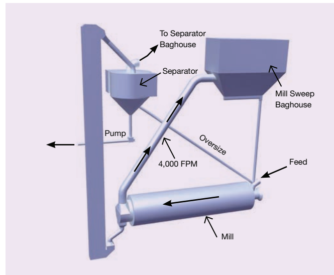
Figure 34. Typical mill sweep arrangement.
