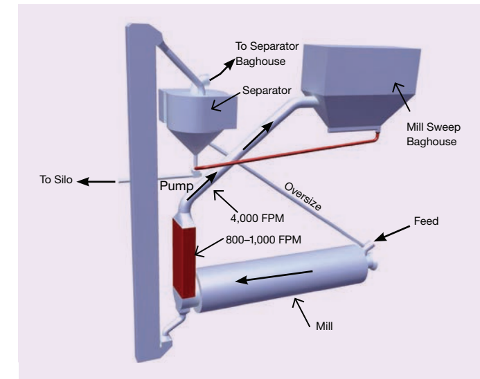
Figure 35. Recommended mill sweep modification.
