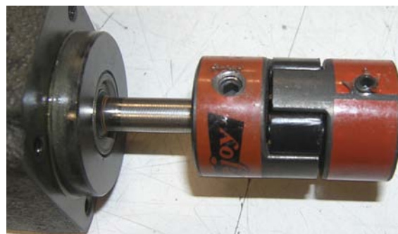
Flexible coupling on pump shaft
