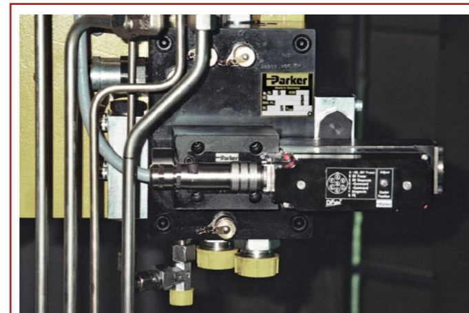
WF Maschinenbau uses Type D3FP*0 valves from Parker Hannifin. These valves feature short switching times of less than six milliseconds, and a frequency response of 200 Hz.
