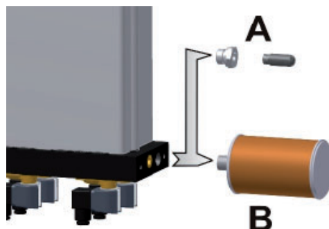
Undo muffler
