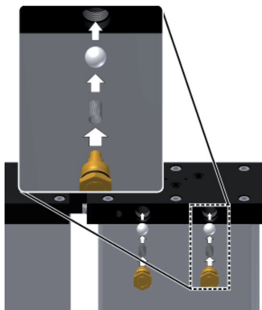
Check valves
