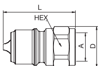
Tarudage
