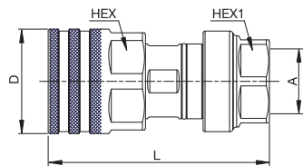
Tarudage - NPTF
