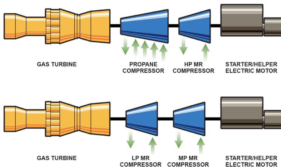
Fig. 1 Air Products C3MR/SplitMR® GT driven refrigerant compression, as used at Cameron LNG
