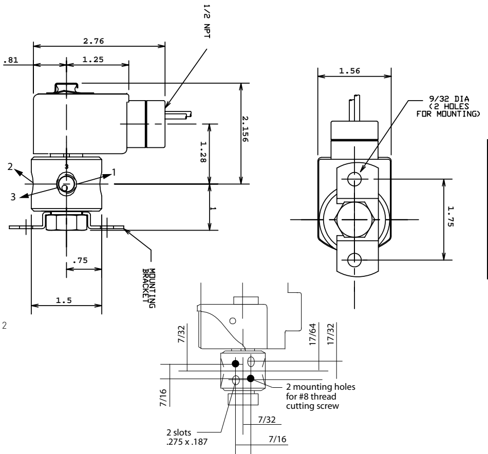
3-Way Normally Open
