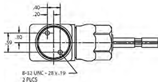
3-Way Universal 30CUxx
