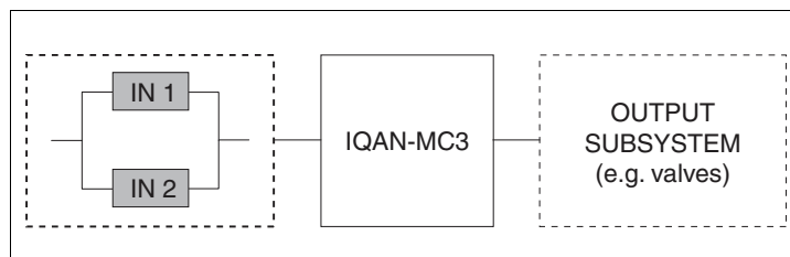
Fully redundant structure.
