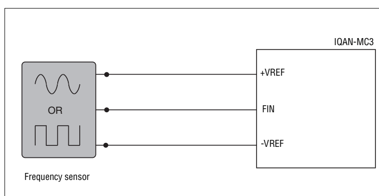
Connecting of frequency sensor to FIN.
