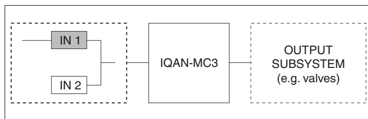
Single structure with monitoring by separate signal.
