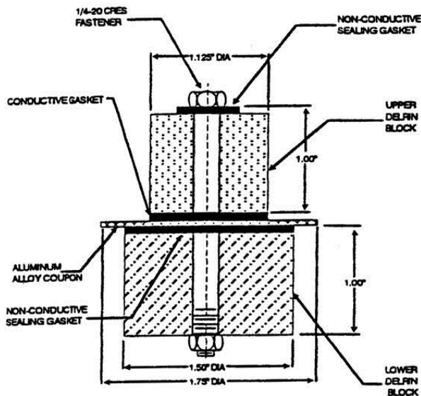
Figure 1 Test Fixture
