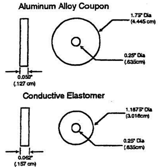
Figure 2 Aluminum Alloy Coupon and Conductive Elastomer
