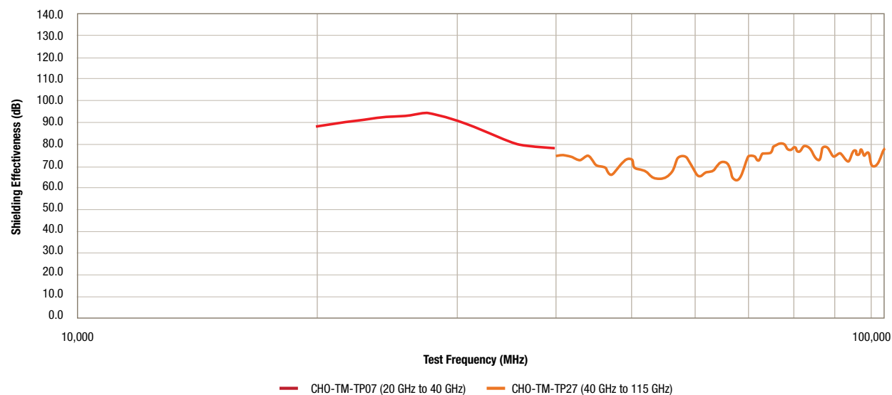
Figure 2 - CHO-SHIELD 2040 Typical Shielding Effectiveness per CHO-TM-TP07 and CHO-TM-TP27
