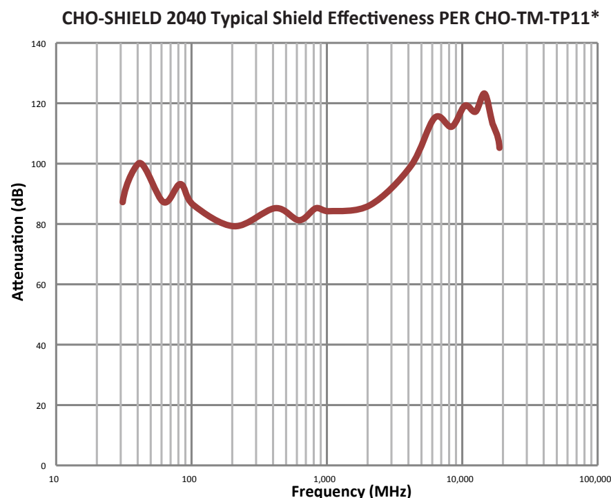
Figure 1 - Typical Shielding Effectiveness
