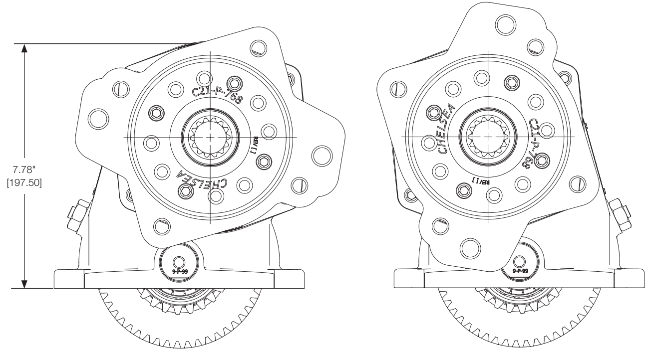
3 Arrangement
