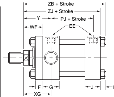
25mm - 80mm Bore Head / Retainer Construction and Rod Extension
