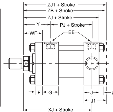
25mm - 80mm Bore Head / Retainer Construction and Rod Extension
