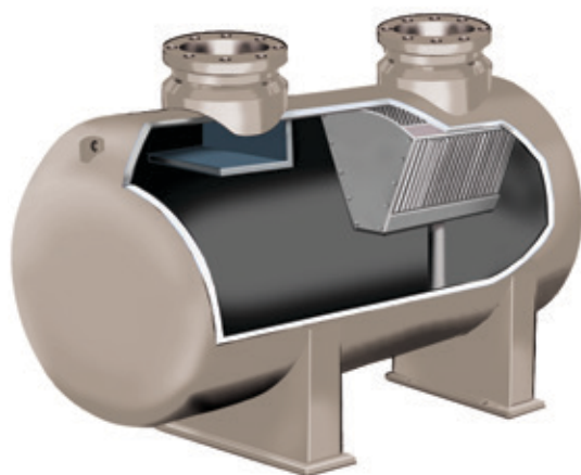
Series 95H-VBANK Scrubber
