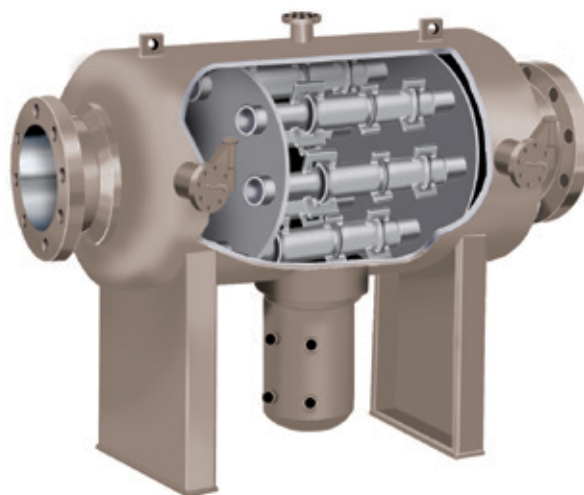
Series 95H-CT Separator
