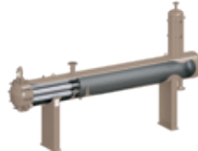
XtreamPhase® Series 110HRXP w/cartridges
