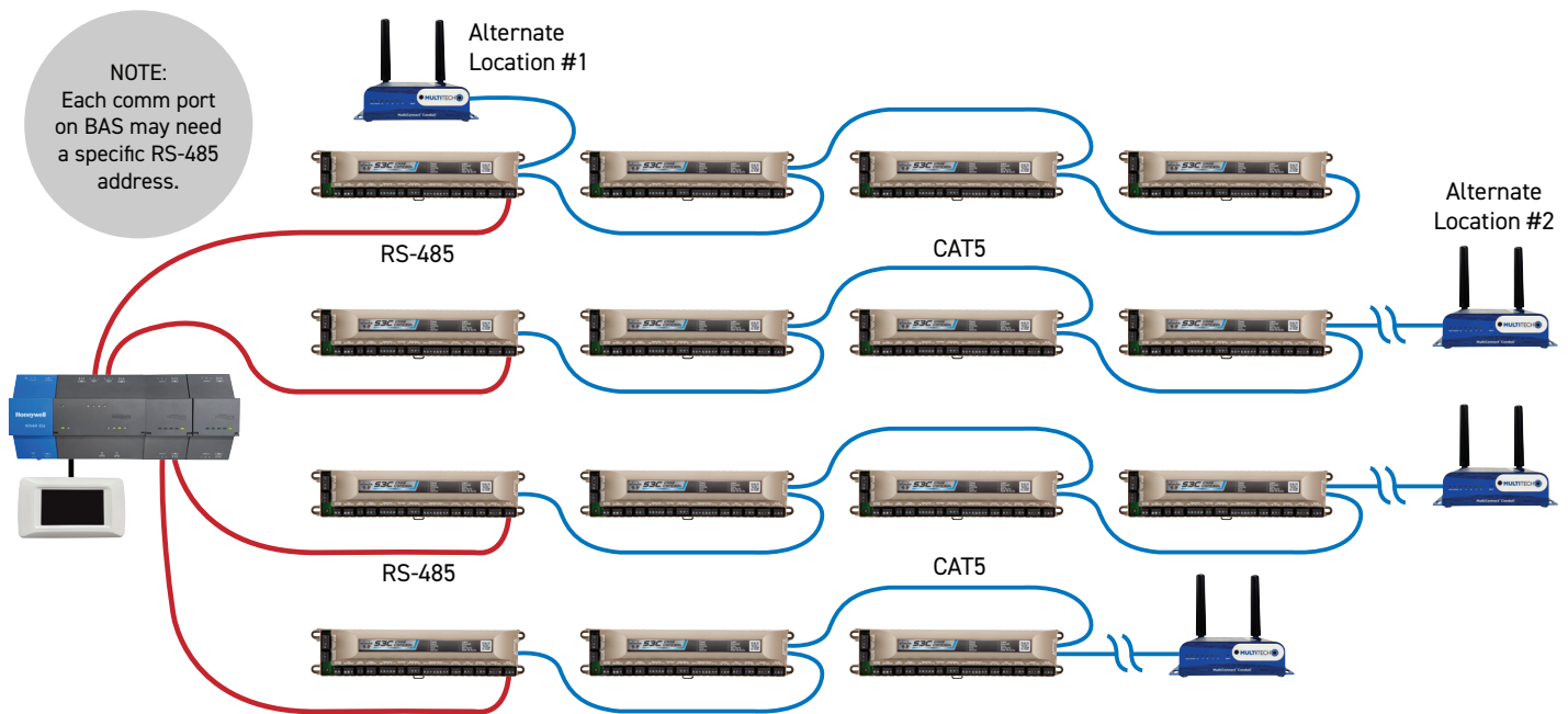
Figure above: Store network showing 4 comm loops into one BAS.
