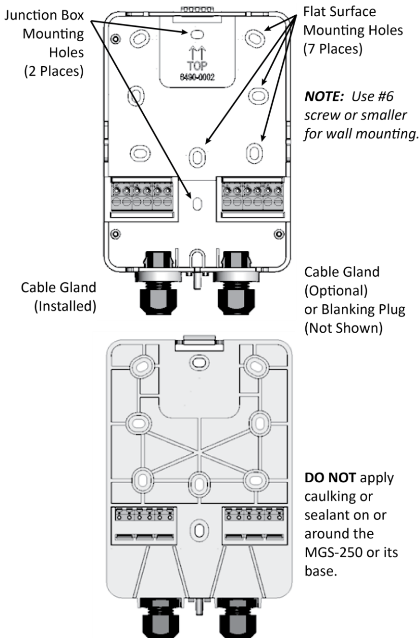
Figure 6. Front and Back Views of 023-0480 Base
