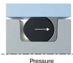
Fig. 10.4 The back-up ring on the non-pressurised side prevents gap extrusion.
