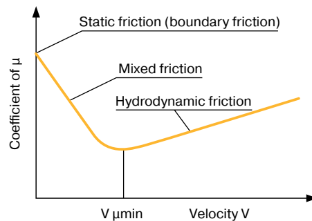
Fig. 8.18 Stribeck curve
