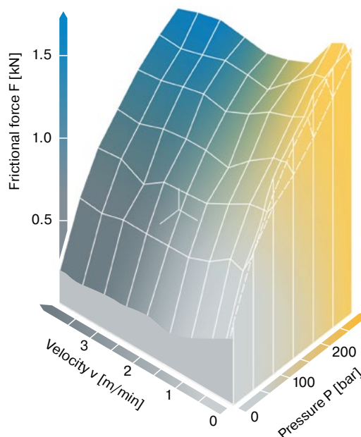
Fig. 8.20 Friction force in relation to pressure and velocity – compact rod seal 90 Shore A
