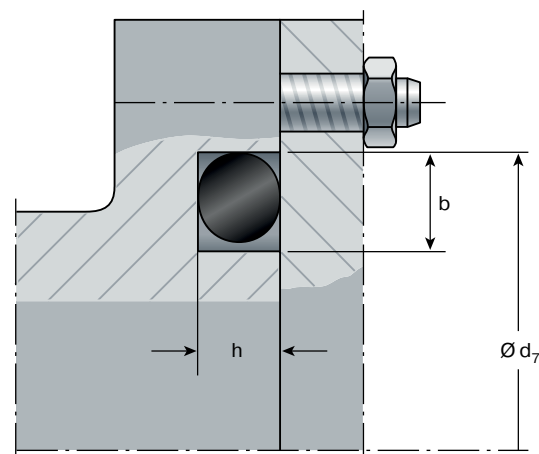
Fig. 3.3 Flange seal – axial compression
