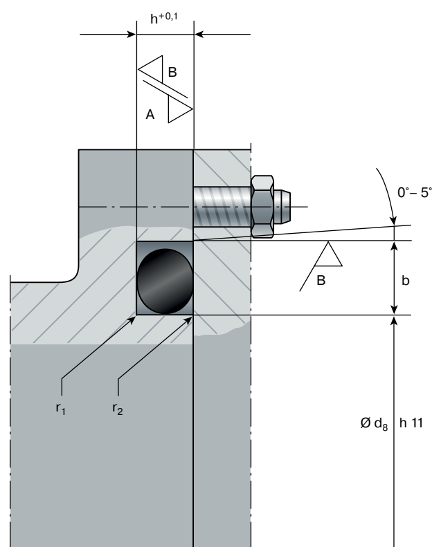
Fig. 2.9 Pressure from outside
