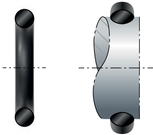
Fig. 8.12 Left: unstretched O-Ring, right: stretched O-Ring
