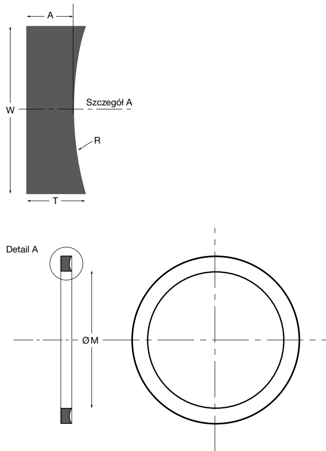
Fig. 4.11 Parbak® back-up ring
