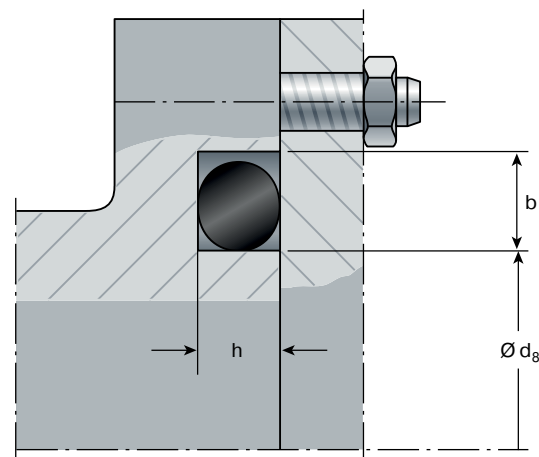
Fig. 3.4 Flange seal – axial deformation
