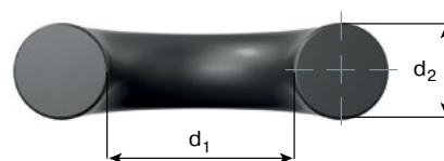
Fig. 2.7 Inner diameter d_1 , cross-section d_2
