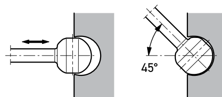
F4 piston-to-shaft locking.
