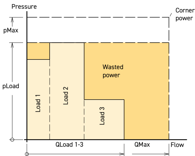
Diagram 1. Constant flow system with a fixed displacement pump.
