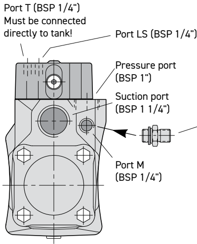
VP1-045/-060/-075 end view (showing ports).
