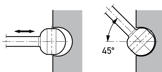
F1 piston-to-shaft locking.
