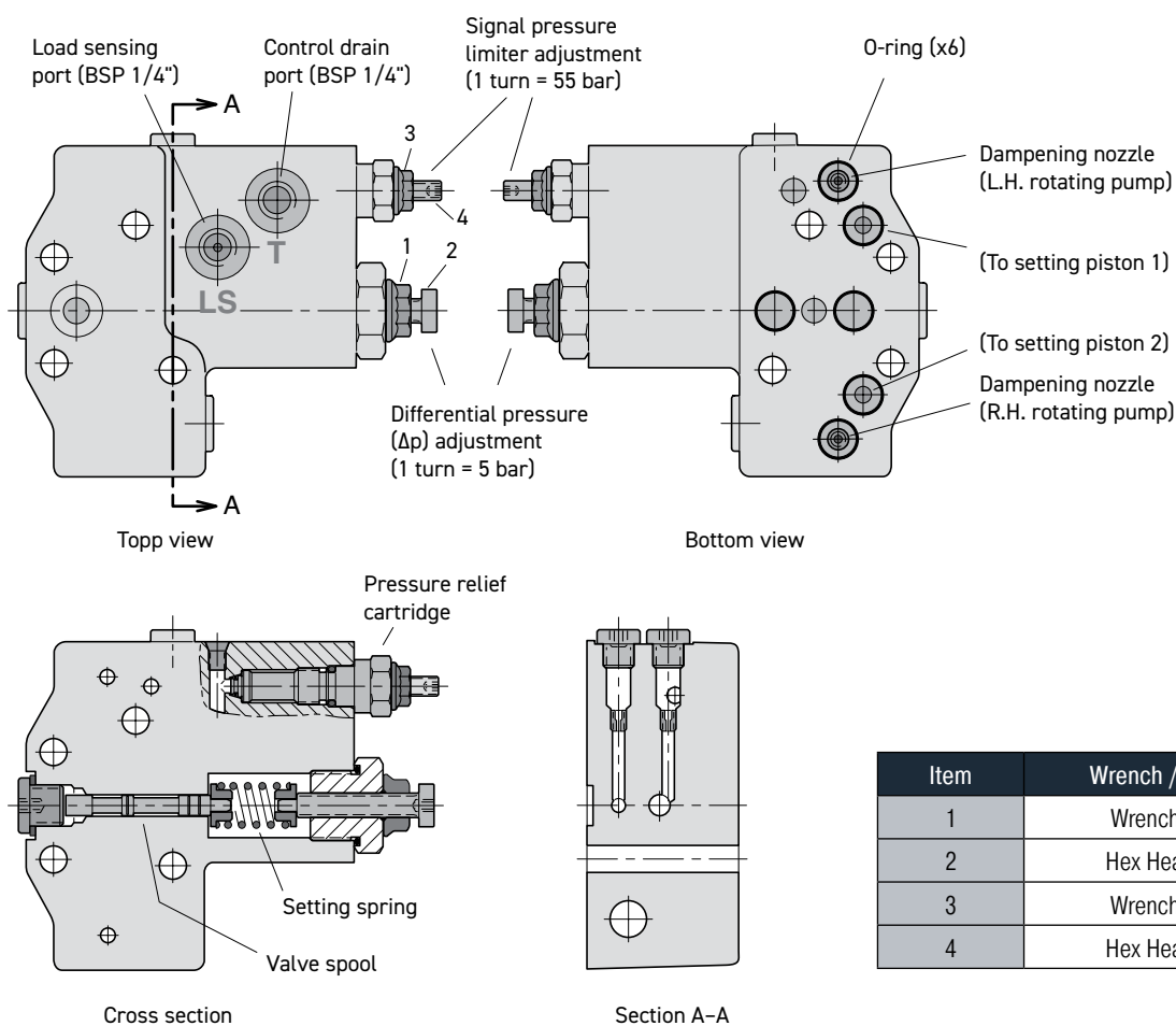
Fig. 2. LS valve block.
