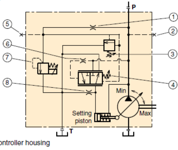
Hydraulic schematic for VP1-095/110/130 EPC2
