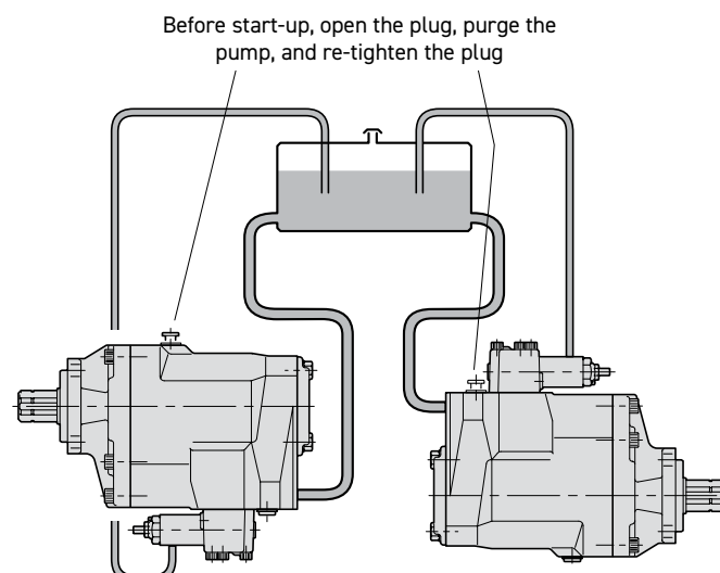
Fig. 8. VP1 should be installed below the reservoir fluid level. Purging should be performed when the pump is connected to the reservoir and the system is filled with fluid.
