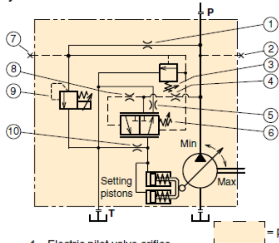
Hydraulic schematic for VP1-045/-060/-075 EPC2
