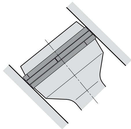
F3 piston with laminated piston ring.
