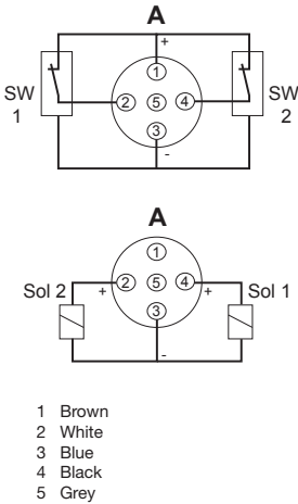
M12 Pinouts for P33
