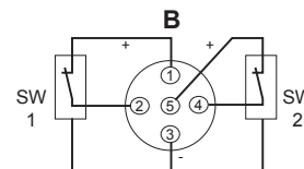
M12 Pinouts for P33
