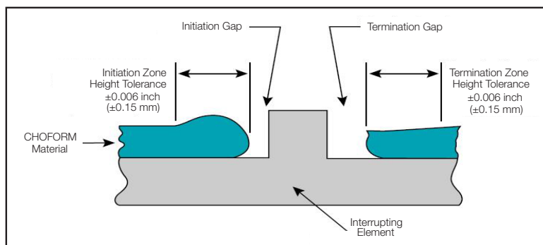
Figure 7-3 Side View Gasket height tolerances
