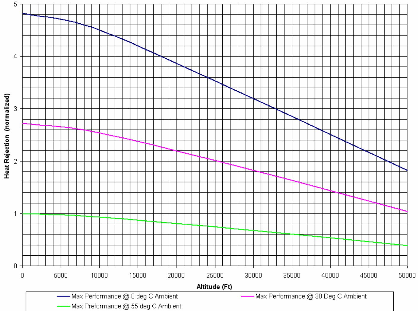
Heat Rejection vs Altitude for Given Ambient Temperature
