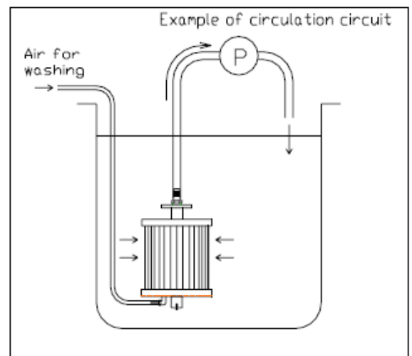
Installation example
