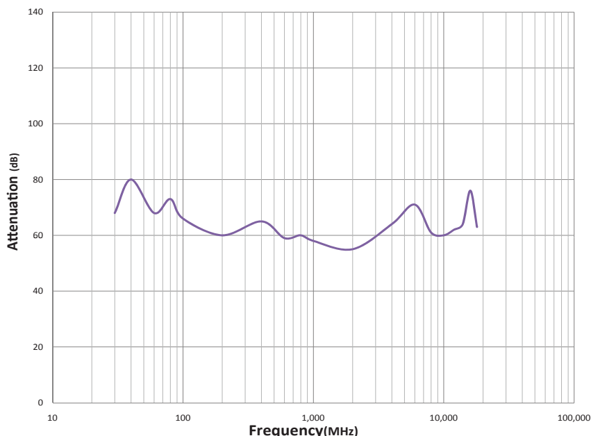
CHO-SHIELD 2044 Typical Shield Effectiveness PER CHO-TM-TP11*
