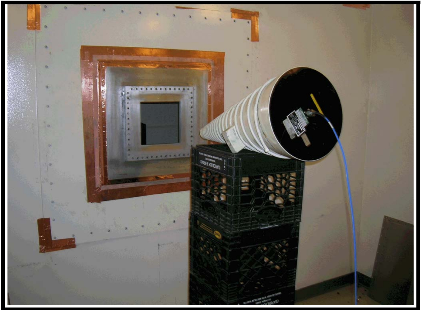
Photograph Description: Basic Thru-Hole Open Reference Setup 200MHz to 1GHz
