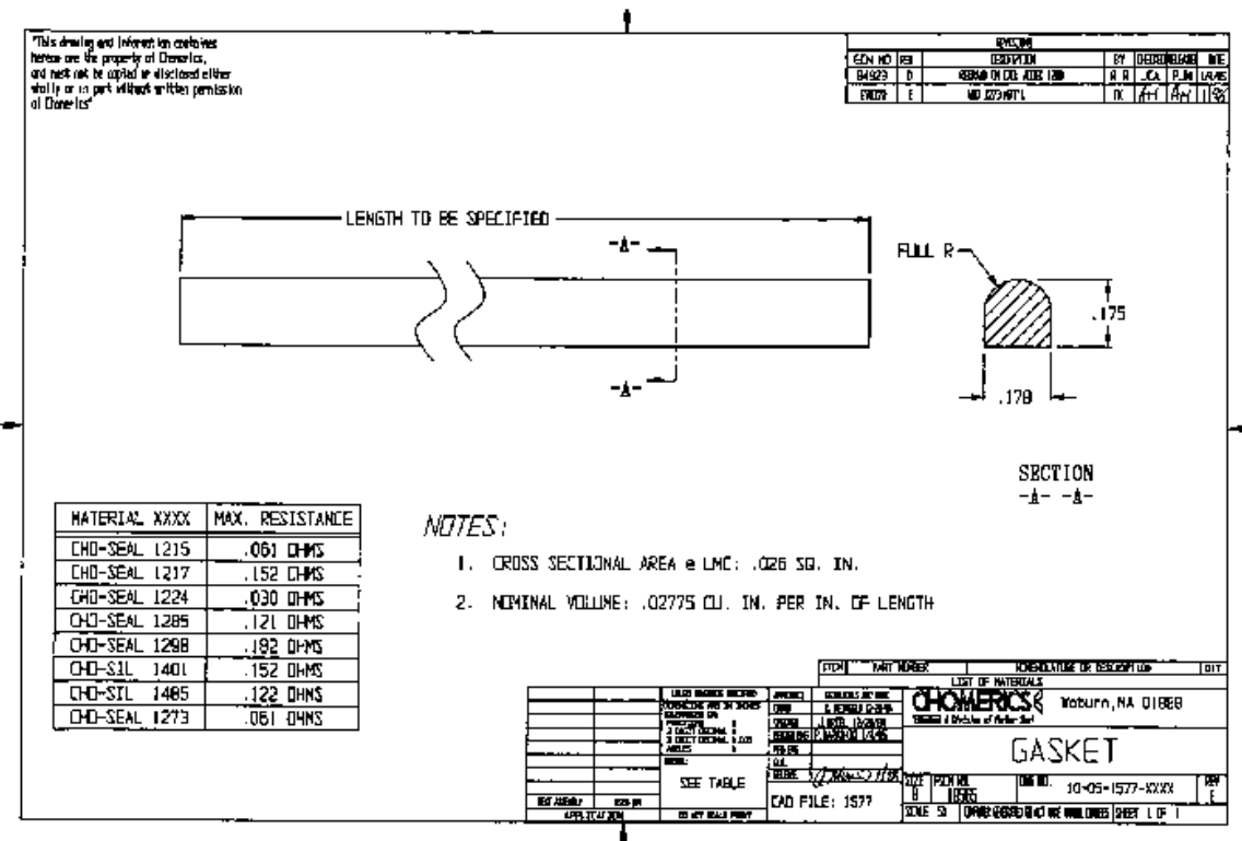
Figure 6 : Drawing of Solid “D” Profile
