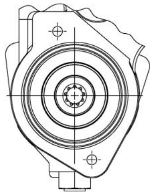
XE Output 5/8"- 9 Tooth Shaft S.A.E. Class "A" 2 Bolt Flange
