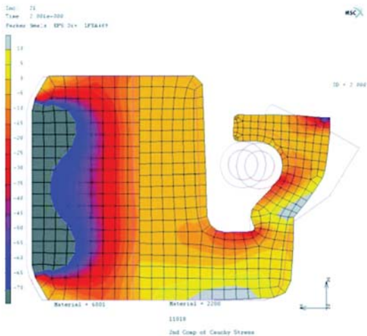
FEA Capability
