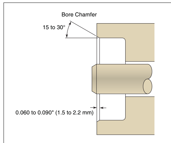
Figure 6-2. Housing Profile
