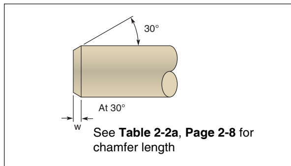
Figure 6-1. Shaft Profile
