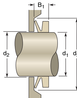
Assembly Dimensions
