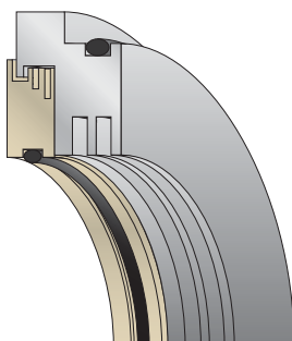
LS Profile
