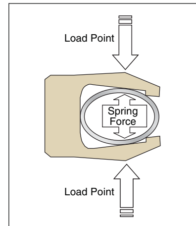
Figure 2-16. Installed State
