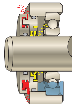
Flow Patterns
