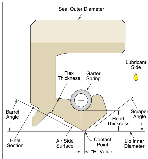
Figure 2-2. Seal Components
