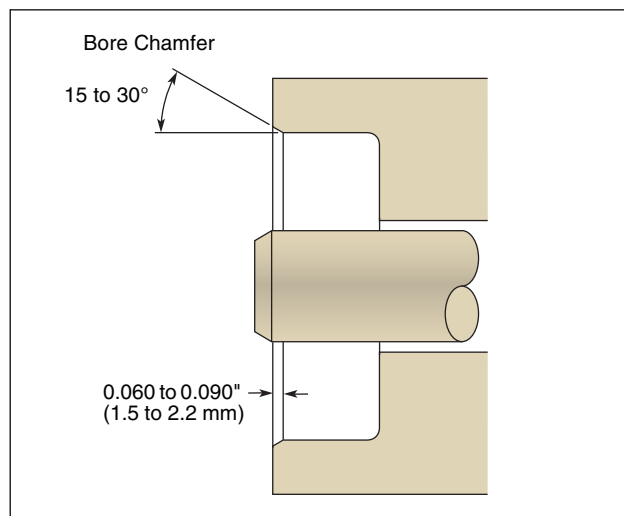
Figure 2-10. Housing Profile
