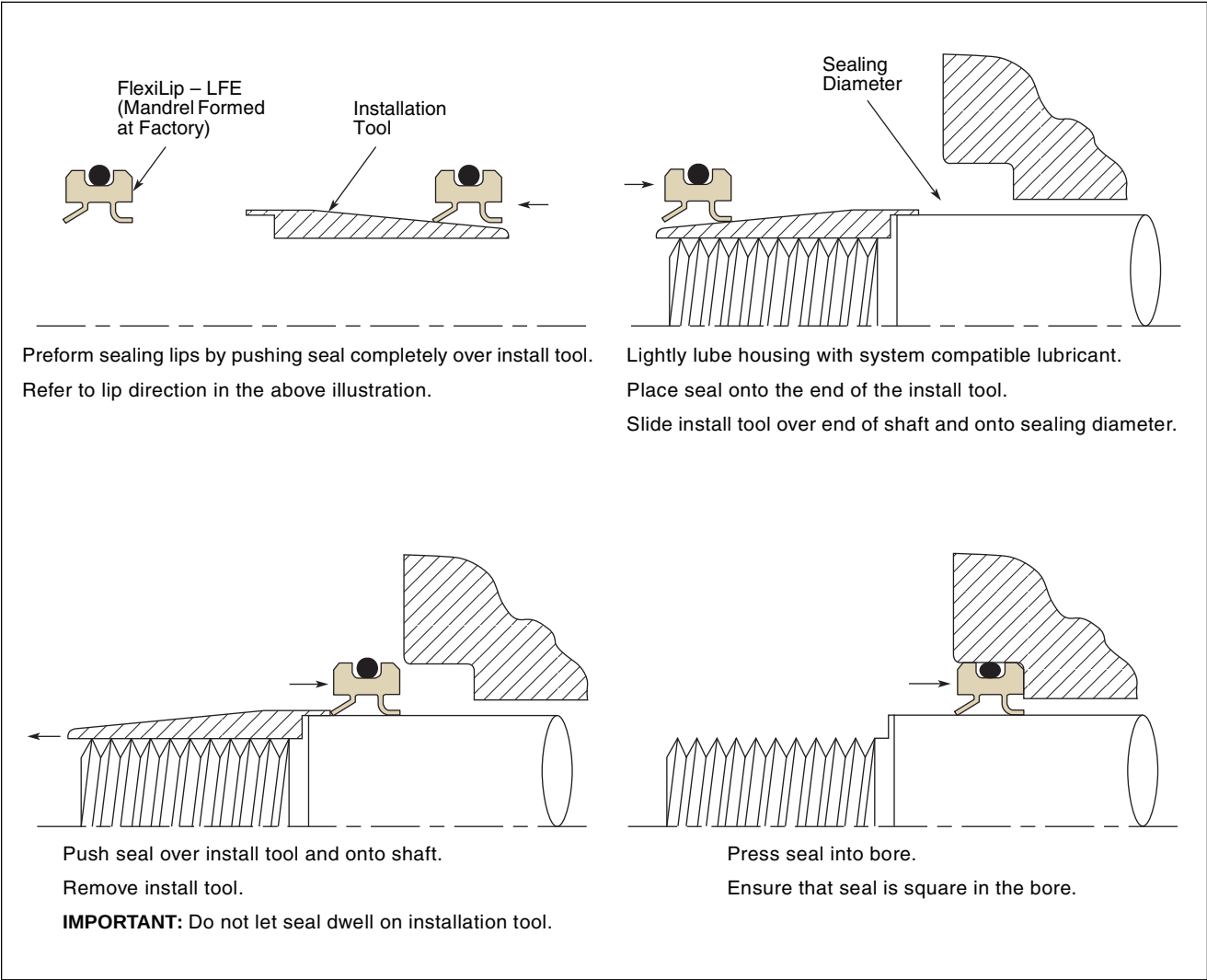
Figure 9-1. FlexiLip Installation
