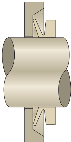
V-Seal L in Assembly
