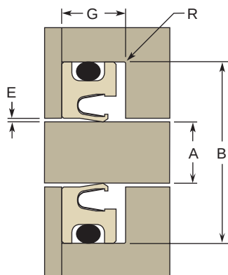
Rotary Seal
